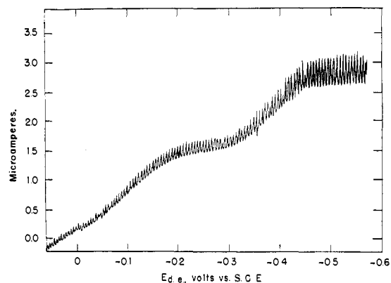
Fig. 1.—Co(III) to Co(II) reduction of 0.001 M trans -isothiocyanatobisethylenediaminecobalt(III) thiocyanate in 0.1 M potassium chloride; one drop 0.1% methyl red added to 25 ml. solution. (Solution about two hours old).
