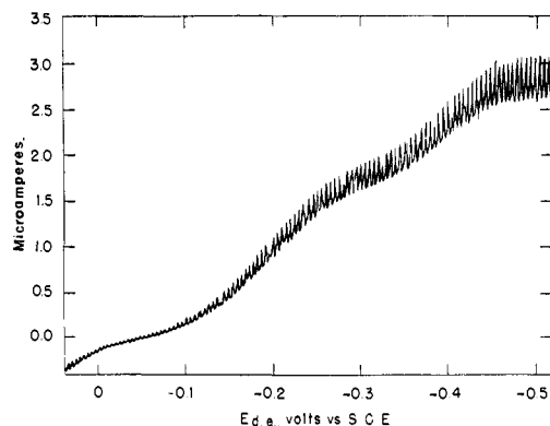
Fig. 3.—Co(III) to Co(II) reduction of 0.001 M trans -nitrobisethylenediaminecobalt(III) nitrate in 0.1 M potassium chloride and 0.002 M sodium bromide.
